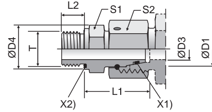
X2) Eoelastic-sealing ED X1) O-ring OR
