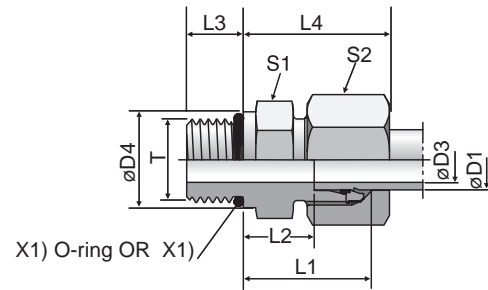
Product images are shown with nuts and sleeves for dimensional allowances only. Part numbers are body level only. See note below product table for details
