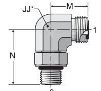
* JJ – Across Wrench Flats
