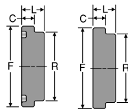
O-ring Face Flat Face
