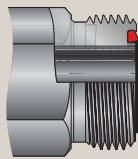
Trap-Seal in half-dovetail groove
