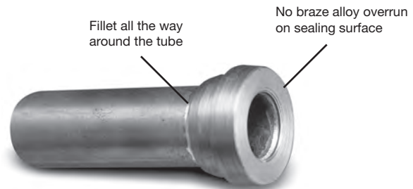
Fig. R24 – Brazed fitting
